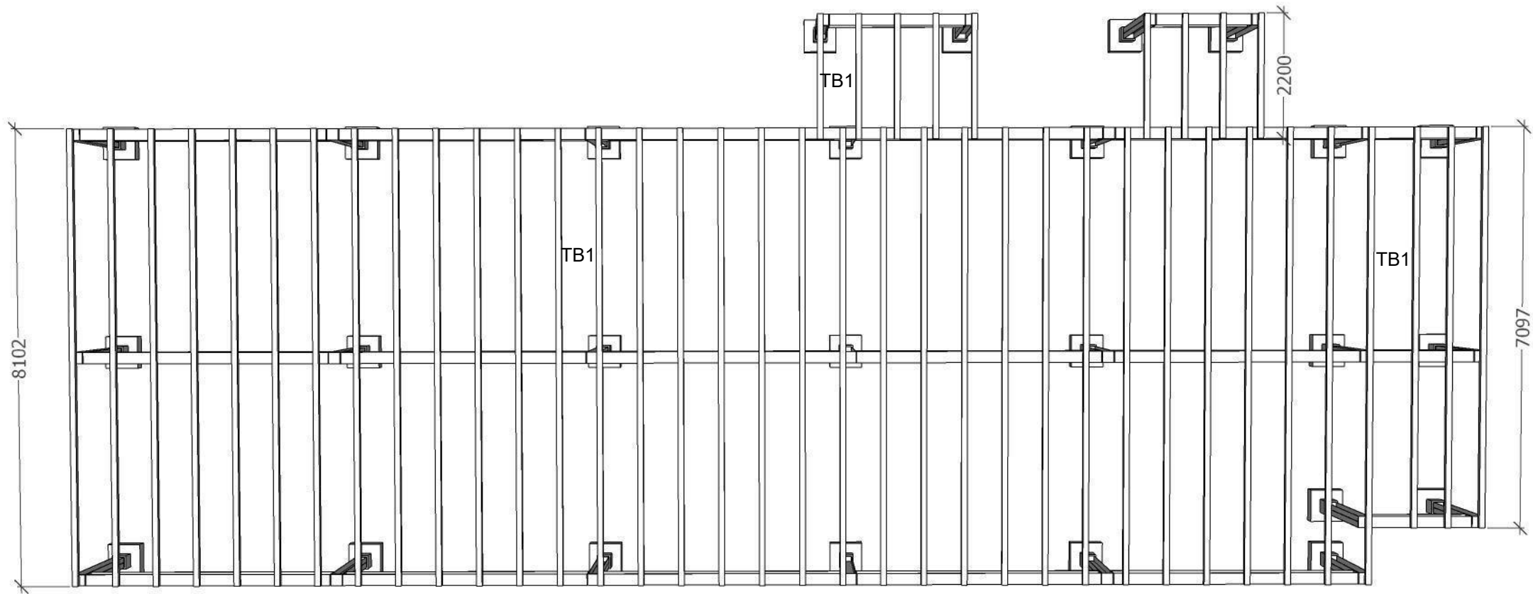
TB1 Floor beams - length
